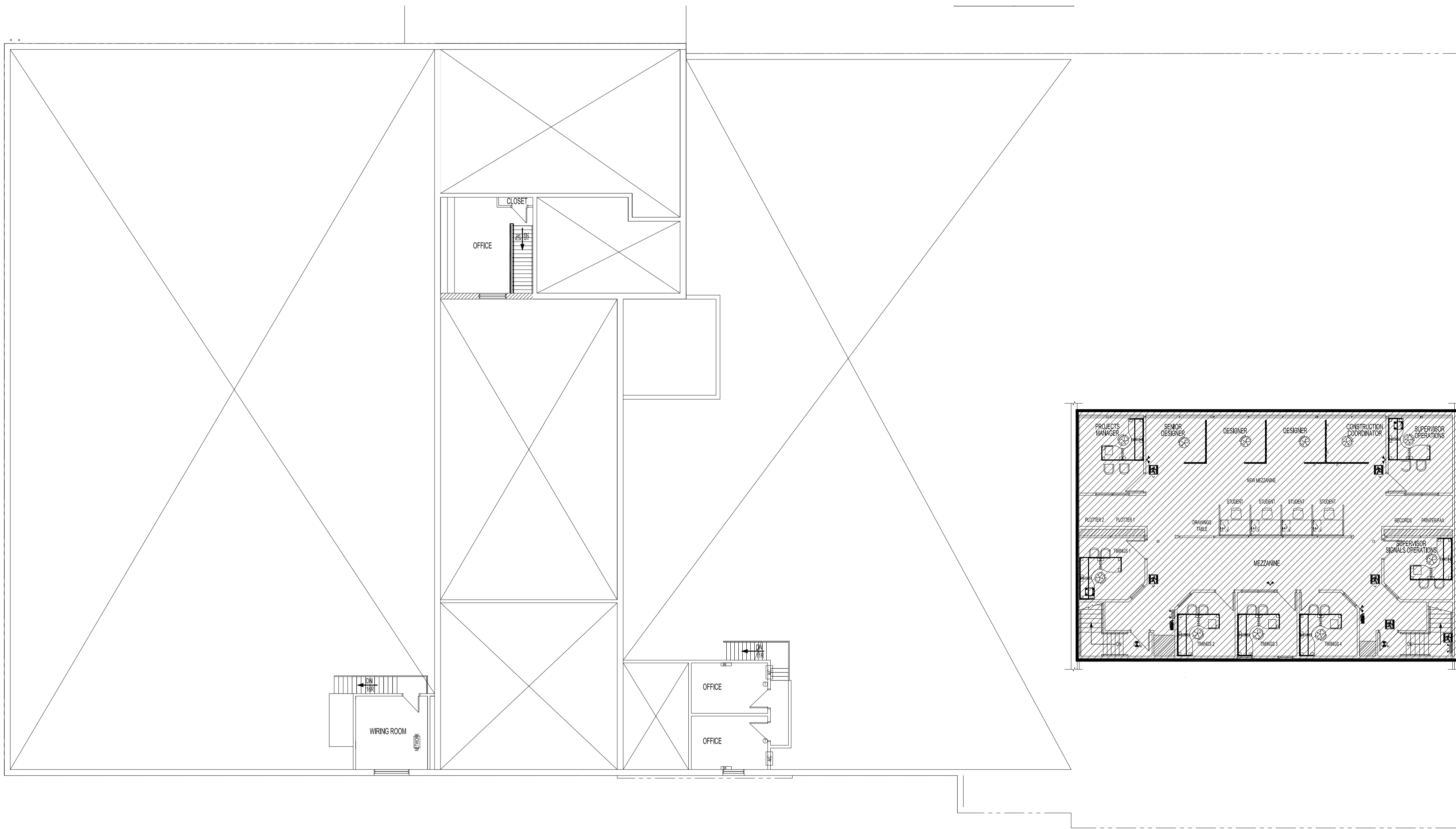
MEZZANINE FLOOR PLAN SCALE: 3/32"=1'-0"
